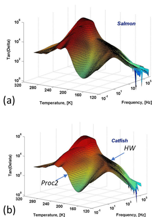
Figure 1 The loss tangent for (a) Salmon and (b) catfish. The measurements were made in the temperature range -100\text{ }^{\circ}\text{C} to 12\text{ }^{\circ}\text{C} and frequency range 10^{-1}\text{ Hz} to 100\text{ kHz} . The main processes are highlighted in (b). 'HW' refers to hydration water around an antifreeze protein.
