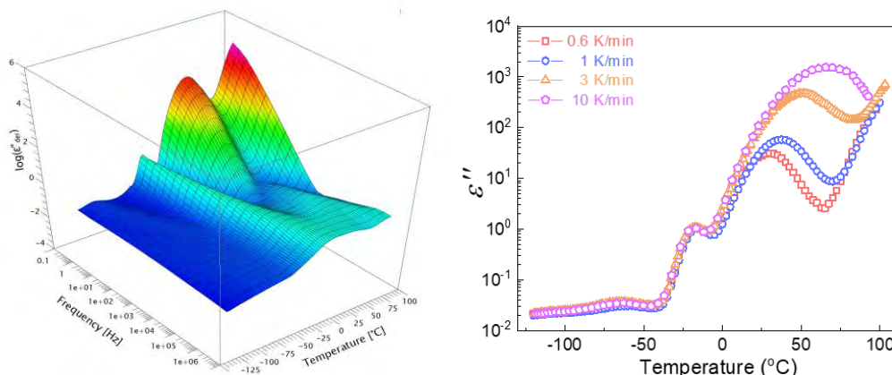
Figure 1. Left: 3D plot of the logarithmic derivative dielectric loss \epsilon''_{der} of the uncured 4F230-2M230 system, Right: Loss \epsilon''(T) at f=100 Hz for 4 different heating rates.
