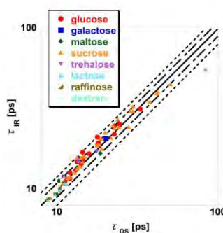
Figure 2. Relaxation time by dielectric spectroscopy, \tau_{DS} , and by SWIR, \tau_{IR} . ( \tau_{IR} = \tau_{DS} (black line), \tau_{DS} \pm 10\% (black chained line), \tau_{DS} \pm 20\% (black dotted line))
