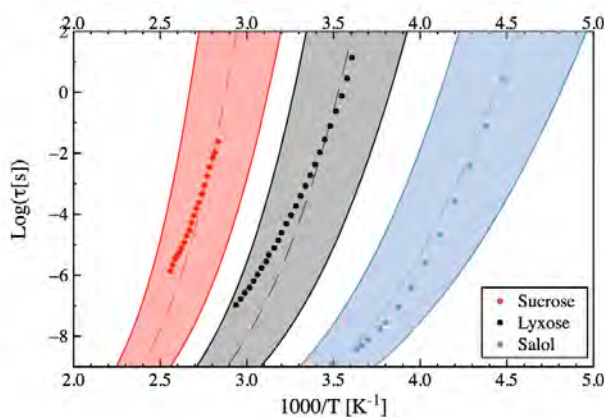
Figure 1. Relaxation map for sucrose, lyxose and salol. Dots represent experimental values measured by broadband dielectric spectroscopy, whereas shaded bands indicate the range of the relaxation times predicted by the joint numerical/theoretical approach proposed here.
