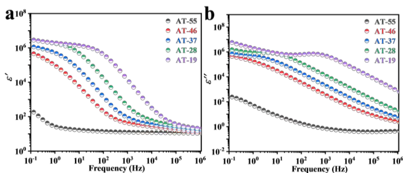
Figure 1. The a) real part and b) imaginary part of permittivity spectra of AT-55, AT-46, AT-37, AT-28 and AT-19 at -40°C.
