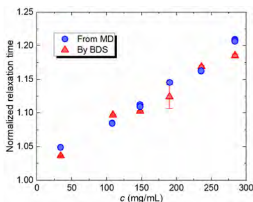
Figure 1. Normalized relaxation time of various concentrations of lysozyme solutions [2].
