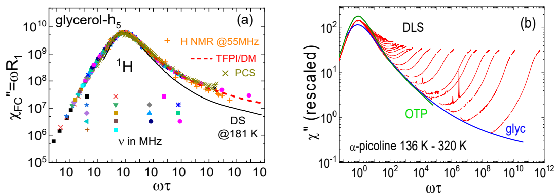
Figure 1. (a) FC 1 H NMR master curves of glycerol-h 5 (colored points); added: single-frequency 2 H NMR (orange), photon correlation spectroscopy (PCS, dark yellow) [3], tandem Fabry-Perot/double monochromator (TFPI/DM, red dashed line) and dielectric spectra (DS, black line), all rescaled. (b) DLS spectra of picoline (red), glycerol (blue) and of o-terphenyl (green) showing different spectral widths.
