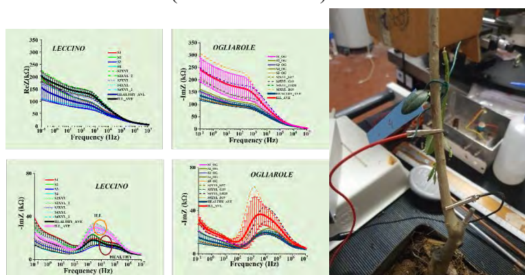
Figure 1. In vivo read outs of the impedances ( Z ) of two olive species (LECCINO and Ogliarola) in healthy and Xylella affected status. The experimental configuration is on the right. The spectra of the affected plants appear modified although symptoms are not yet present. Differences in the magnitude of modification is observed due to the higher resistance of LECCINO with respect to OGLIAROLA.
