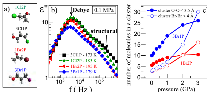
Figure 1. The chemical structures of the studied alcohols (a). Comparison dielectric loss spectra at ambient pressure for studied alcohols characterized by the same relaxation times (b). The evolution of the average number of molecules in hydrogen-bonded and halogen clusters with pressure (c).
