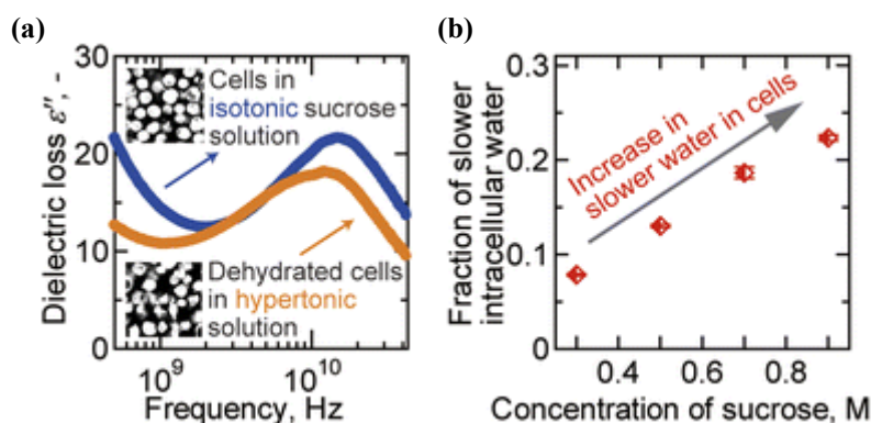
Figure 1. (a) The dielectric loss of Jurkat cells suspended in aqueous sucrose solution. (b) The fraction of slower intracellular water. [2]
