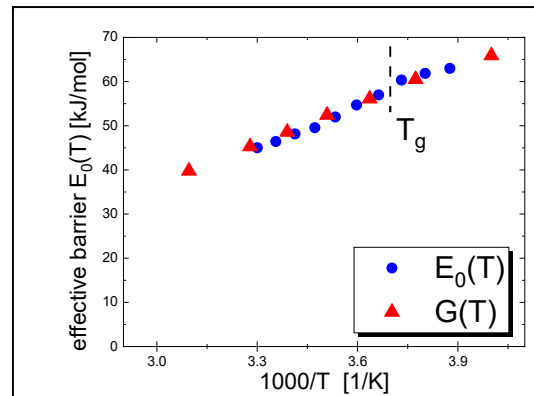
Figure 1. Temperature dependence of the estimated energy barrier for ion transport in polymerized ionic liquid with mobile TFSI ion follows well the temperature dependence of the shear modulus. Data from [1].
