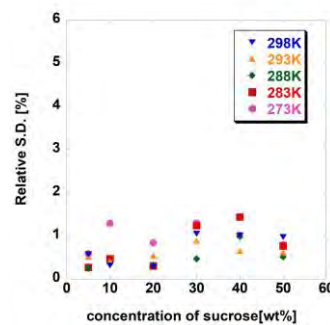
Figure 3. Relative standard deviation to concentration in two-dimensional distribution measurements of sucrose [4]
