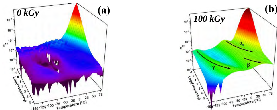
Figure 1. 3D relaxation map of virgin (a) and irradiated (b) LLDPE at 100 kGy measured by Broadband Dielectric Spectroscopy.
