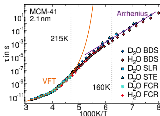
Figure 1: Correlation times of water in silica pores with diameter of 2.1 nm from BDS and various NMR methods [1], where BDS data for H 2 O is taken from [3].
