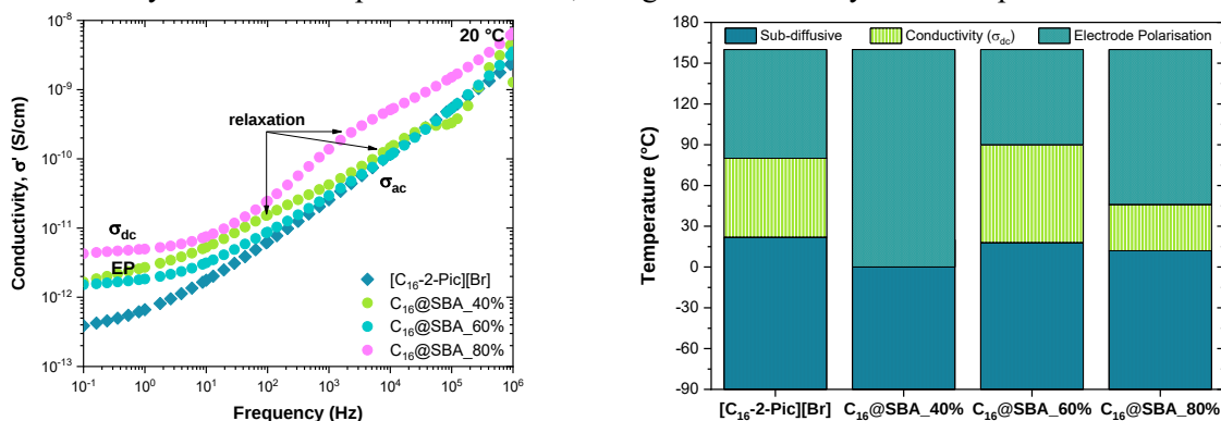
Figure 1. Comparison between the real conductivity spectra at 20^\circ\text{C} for [C_{16}\text{-}2\text{-Pic}][\text{Br}] and the three composites, which is also schematised over a wide T -range on the right-side plot.
