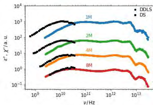
Figure 1. Comparison of dielectric loss (black squares) and DDLS susceptibility (colored circles) of aqueous lithium chloride solutions (from top to bottom: 1 molar to 8 molar) at 263 K.
