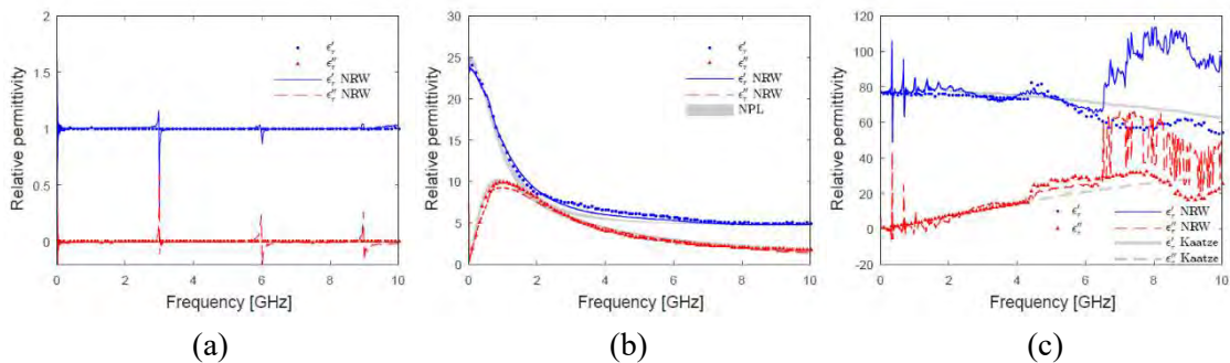
Figure 1. Complex permittivity of (a) air, (b) ethanol, and (c) water obtained using the proposed method, NRW method, and found in the literature[2][3].
