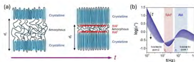
Figure 1. (a) Graphical representation of changes in the domain spacing during crystallization. (b) Dielectric loss curves during isothermal measurements at T_c = 402 \text{ K} . The Restricted amorphous fraction (RAF) emerges following long equilibration times [4].
